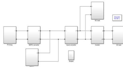
Fig.2. Simulation circuit
