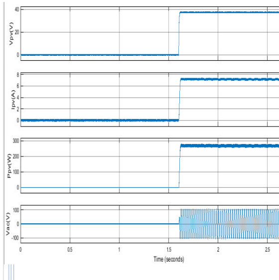
Fig.10. MPPT and inverter waveform Without FLC.
