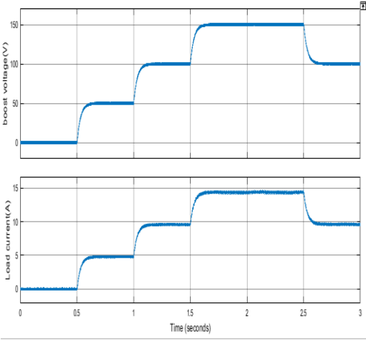
Fig.8. BOOST CONVERTER STEP REFERENCE without fuzzy
