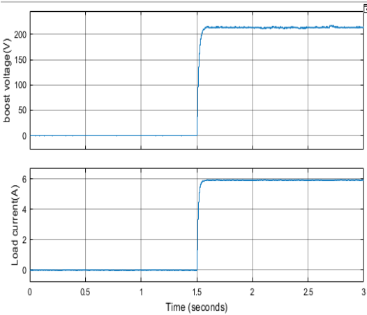
Fig.7. BOOST CONVERTER using with fuzzy
