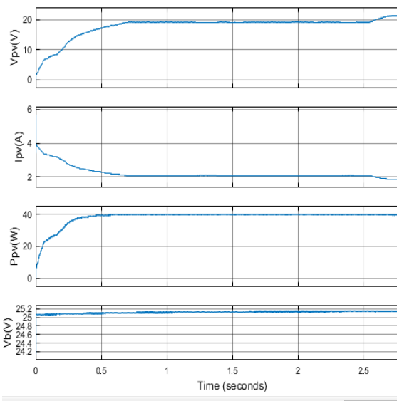
Fig.4. MPPT without fuzzy
