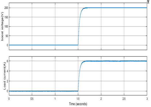
Fig.6. BOOST CONVERTER using without fuzzy
