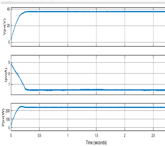
Fig.3. SEPIC converter output
