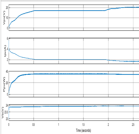
Fig.4. MPPT without fuzzy
